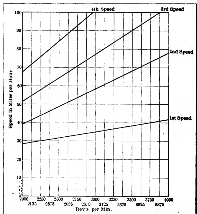
Fig. 2.—Diagram showing the speed in miles per hour of a car fitted with a 3.3-inch bore motor
